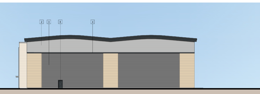
SOUTHERN ELEVATION
