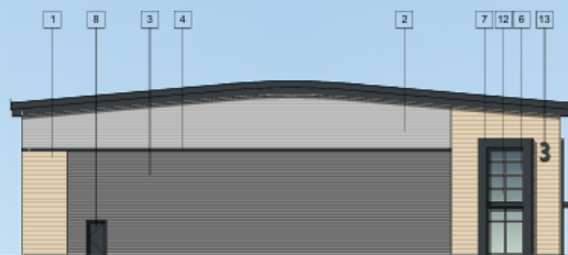
EAST ELEVATION
